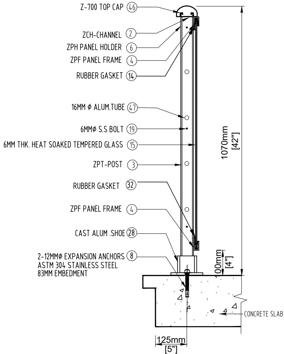
CROSS SECTION TYPE - 9 ALUM.PIPE & GLASS RAILING TOP CAP, TOP MOUNTED
