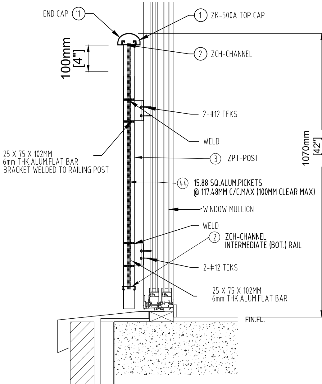
CROSS SECTION TYPE-18C ALUMINUM COMMERCIAL FRENCH BALCONY
