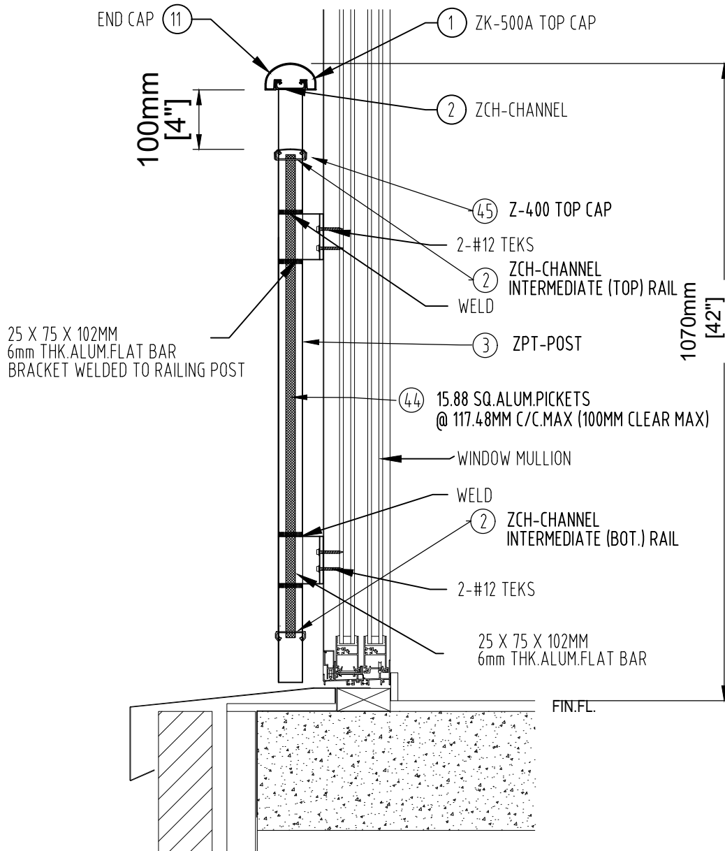
CROSS SECTION TYPE-18B ALUMINUM COMMERCIAL FRENCH BALCONY
