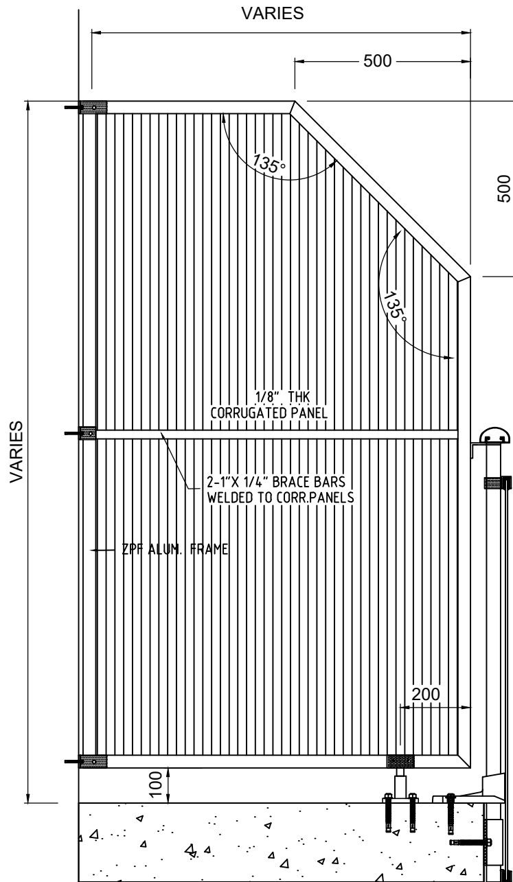
DIVIDER TYPE-4 CORRUGATED ALUM. PANEL
