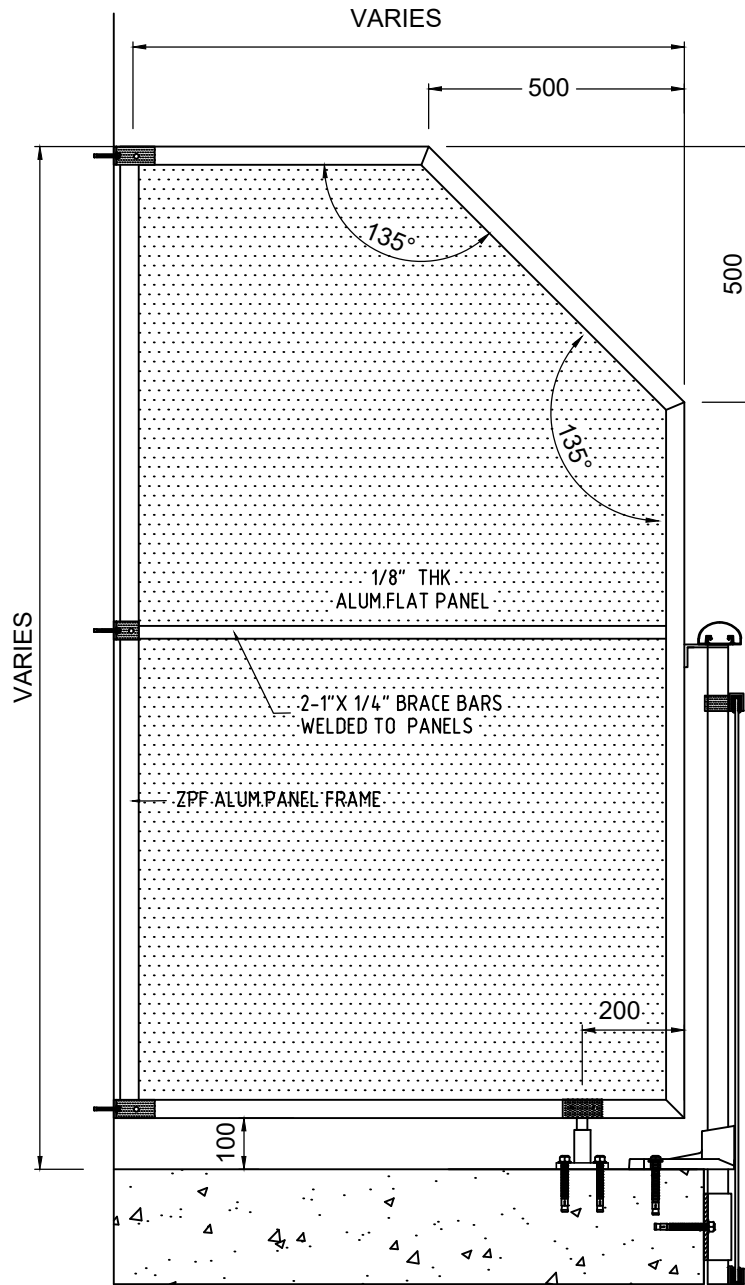
DIVIDER TYPE-3 1/8" THK. ALUM. FLAT PANEL
