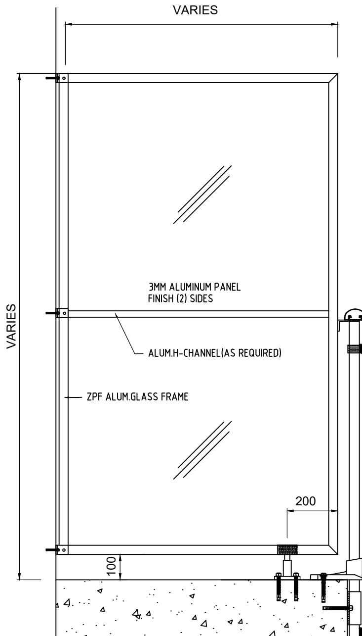
DIVIDER TYPE-2B ALUM.GLASS PANEL
