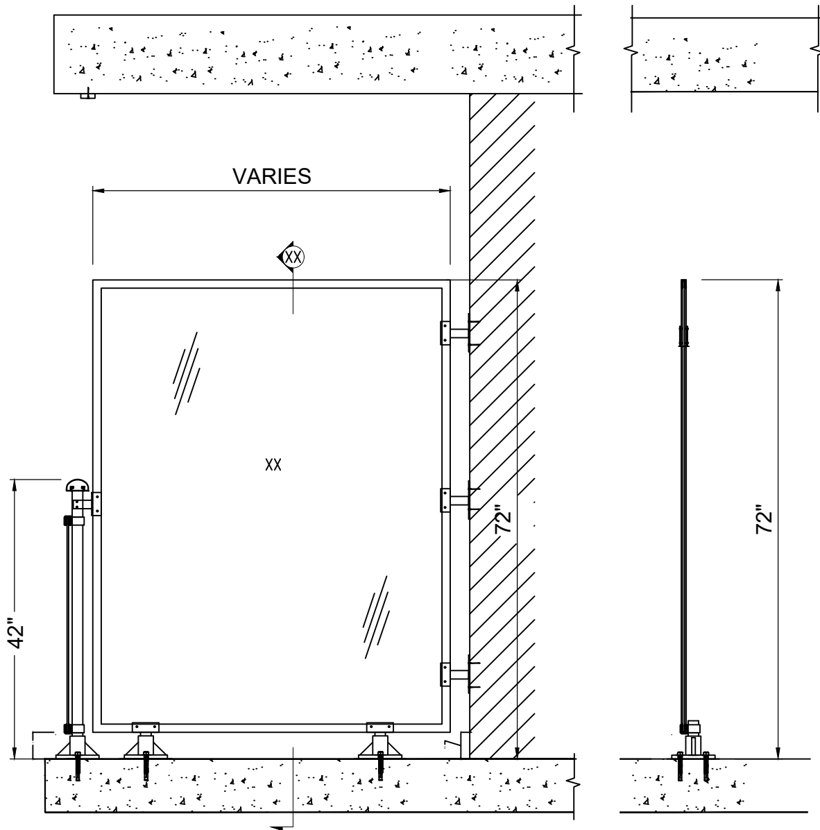
SECTION "E"
